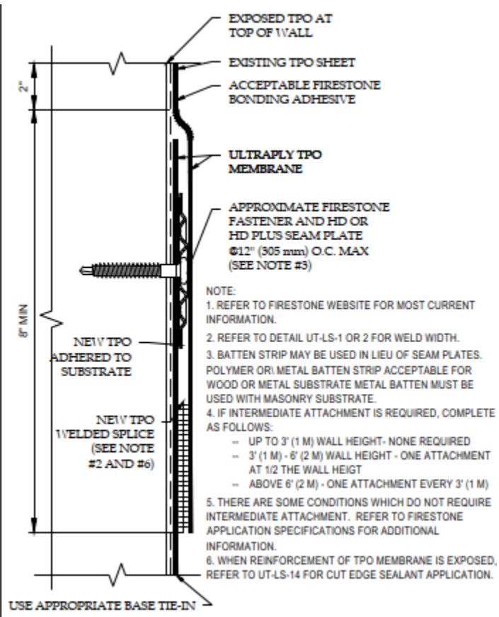
DETAIL W1- WALL REPAIR DETAIL
